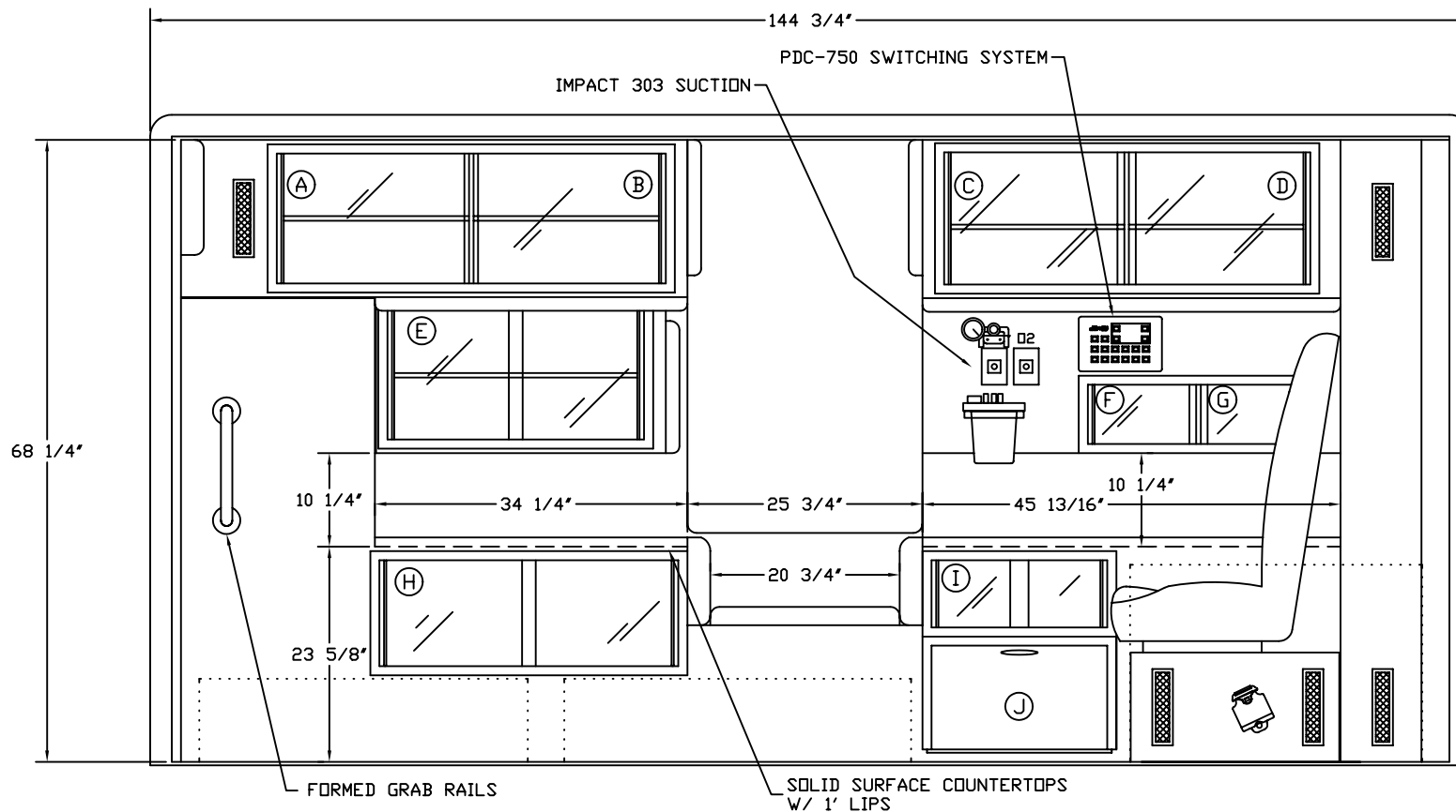
STANDARD LEFT SIDE
