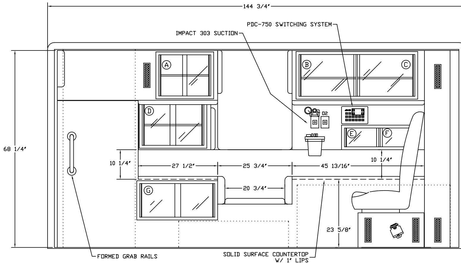
LEFT SIDE W/ DOUBLE D1 EXTERIOR COMP..
