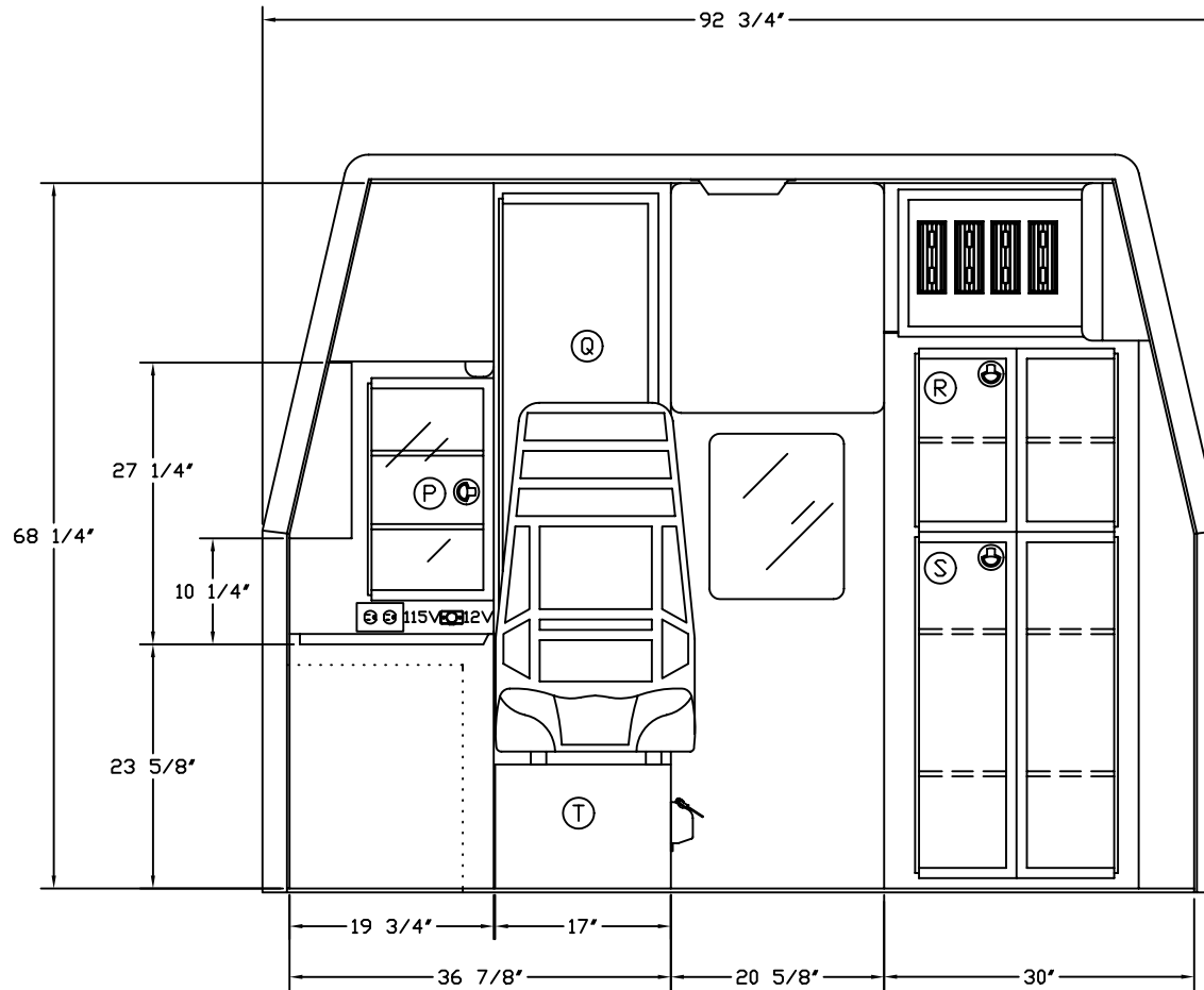
STANDARD FRONT VIEW
