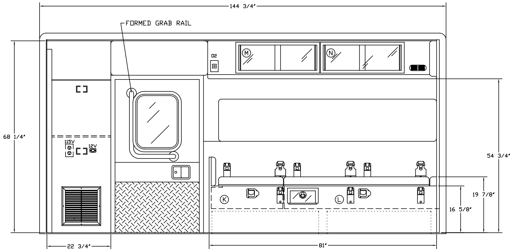
RIGHT SIDE W/ BANDAGE CABINET
